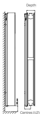
Type 20 Vertical Flat radiator
