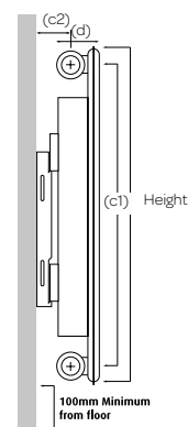
Type 11 Single Convector
