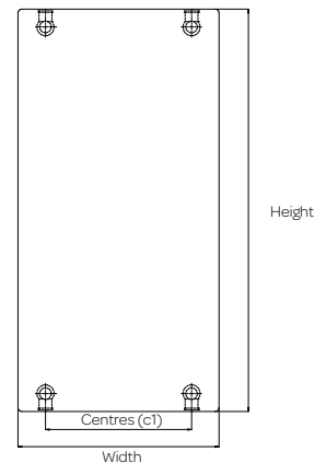
TYPE 20 Double Panel (With Side Panels)
