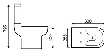
Close Coupled WC
