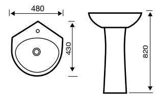
480mm Corner Basin
