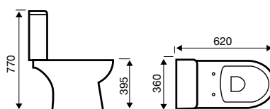
Close Coupled WC
