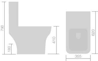
W355 H790 D620 £269
