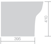
F01884 / F01888 Back to wall WC inc. soft close seat
