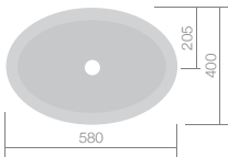
F07400 600mm Countertop wash basin (no overflow) W580 H150 D400 £425
