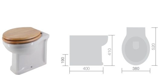
F01893 Back to wall pan £132 W385 H410 D520
