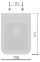
W355 H365 D490 £205
