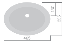
F04408 Lily 465mm basin W465 H180 D335 £95
