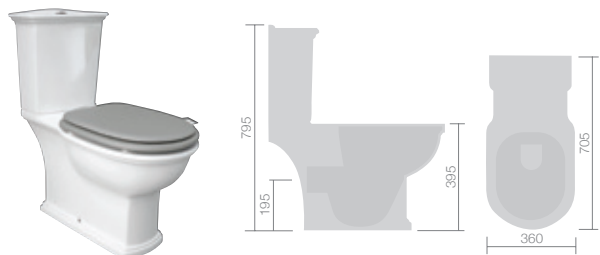
F04486 / F04484 / F04489 WC inc. white wooden soft close seat W360 H795 D705 £462
