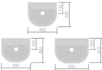
F04356 Compact Slimline 400mm 1TH LH W400 H175 D325 £142 F04357 Compact Slimline 400mm 1TH RH W400 H175 D325 £142 F04358 Compact 450mm 1TH LH W450 H185 D360 £168 F04359 Compact 450mm 1TH RH W450 H185 D360 £168 F04360 Compact 450mm 2TH W450 H185 D360 £168 F04373 Compact 550mm 1TH W550 H195 D415 £168 F04374 Compact 550mm 2TH W550 H195 D415 £168
