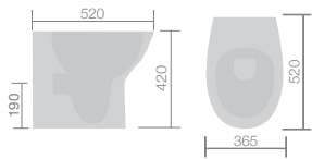
F04415 Back to wall WC inc. soft close seat W365 H420 D520 £226
