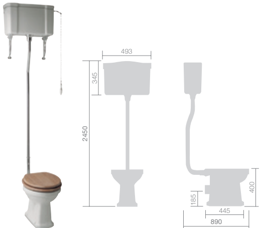
F01898 / F01896 / F01238 High level WC W493 £615
