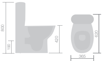
F04414 Flush to wall WC inc. soft close seat W365 H800 D620 £326
