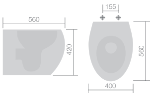
F07405 Back to wall WC inc. soft close seat W400 H420 D560 £971
