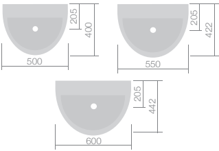
W500 H160 D400 £90 W550 H160 D422 £95 W600 H160 D442 £100 £79 £79
