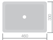
F02600 Square basin W460 H190 D330 £95
