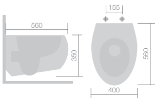
F07404 Wall hung WC inc. soft close seat W400 H350 D560 £861
