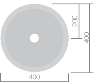
F04384 Emma 400mm basin W400 H215 D400 £110 F04385 Overflow kit £30
