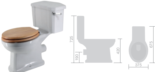
F01895 / F01894 Standard WC £237 W460 H725 D675
