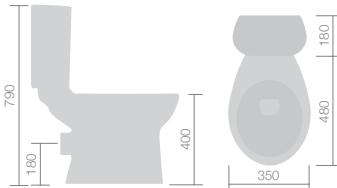
F04315 WC inc. seat F04315 / F04318 WC inc. soft close seat
