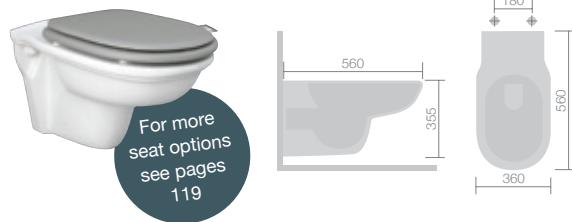
F04490 / F04489 Wall hung WC inc. white wooden soft close seat W360 H355 D560 £290
