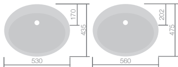
F04406 Jessica 530mm basin 1TH W530 H230 D435 £100 F04407 Jessica 530mm basin 2TH W530 H230 D435 £100 F04410 Maria 560mm basin 1TH W560 H210 D475 £116 F04411 Maria 560mm basin 2TH W560 H210 D475 £116
