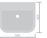
F04458 Series 600 500mm inset basin 1TH W500 H190 D425 £116 F04459 Series 600 500mm inset basin 2TH W500 H190 D425 £116
