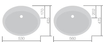
F04406 Jessica 530mm basin 1TH W530 H230 D435 £95 F04407 Jessica 530mm basin 2TH W530 H230 D435 £95 F04410 Maria 560mm basin 1TH W560 H210 D475 £110 F04411 Maria 560mm basin 2TH W560 H210 D475 £110
